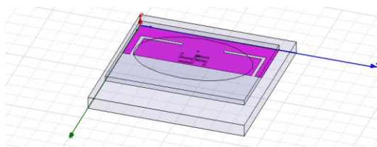
Fig. 1 L-slot design
