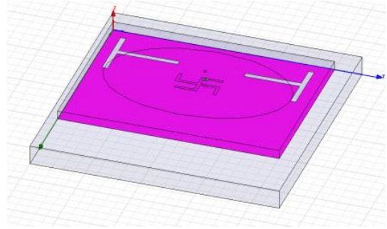
Fig. 2 T-slot design
